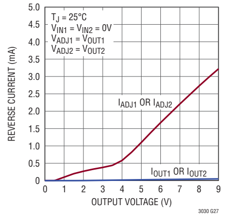
Reverse Current
